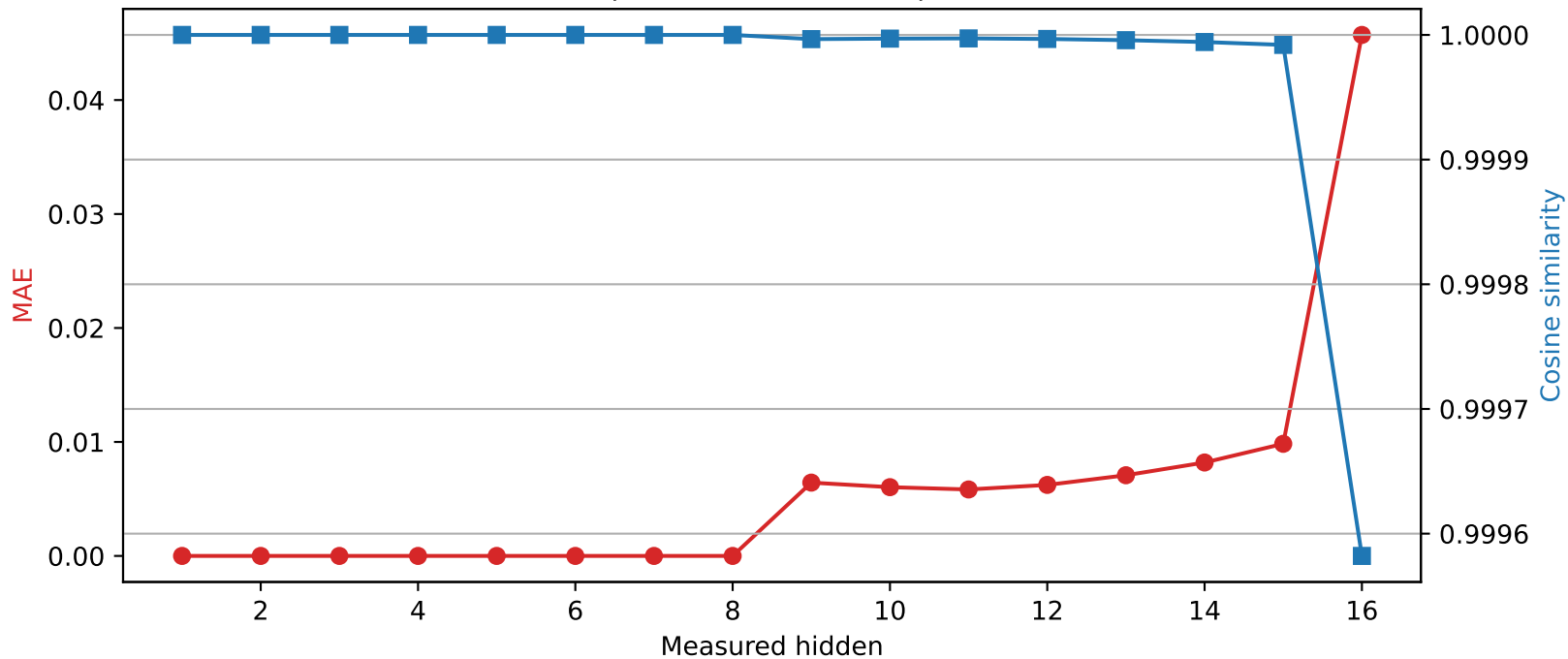
Llama-3.2-1B | Quantized layer 8 | float64 \rightarrow int8
