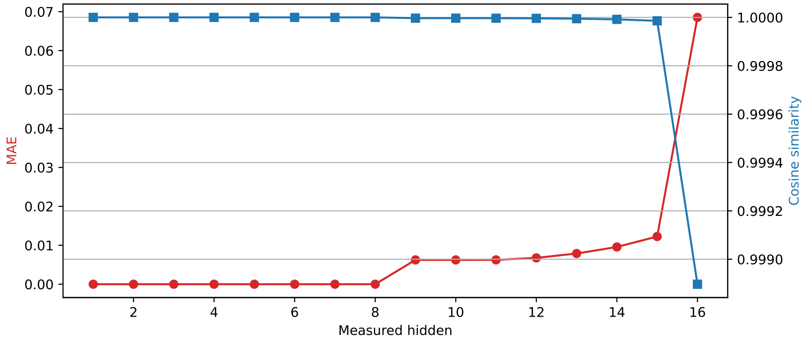
Llama-3.2-1B | Quantized layer 8 | float64 → int8
