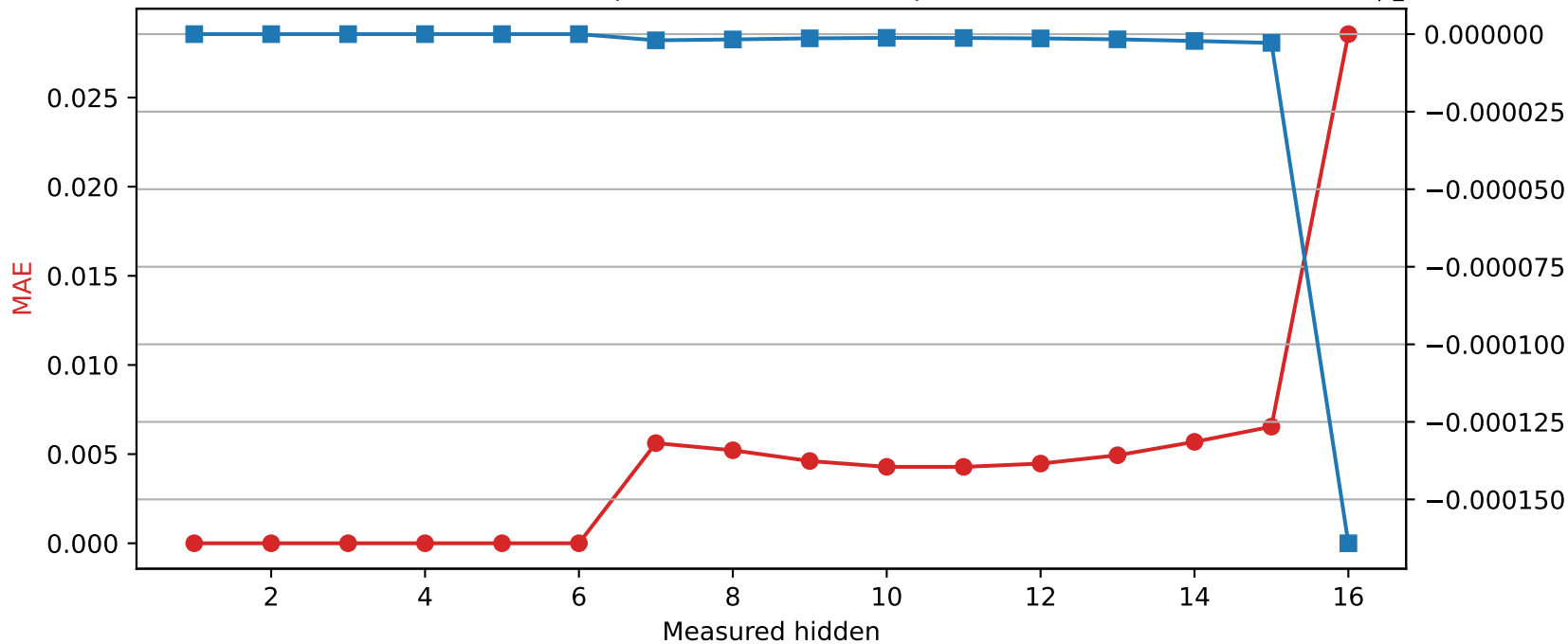
Llama-3.2-1B | Quantized layer 6 | float64 → int8
