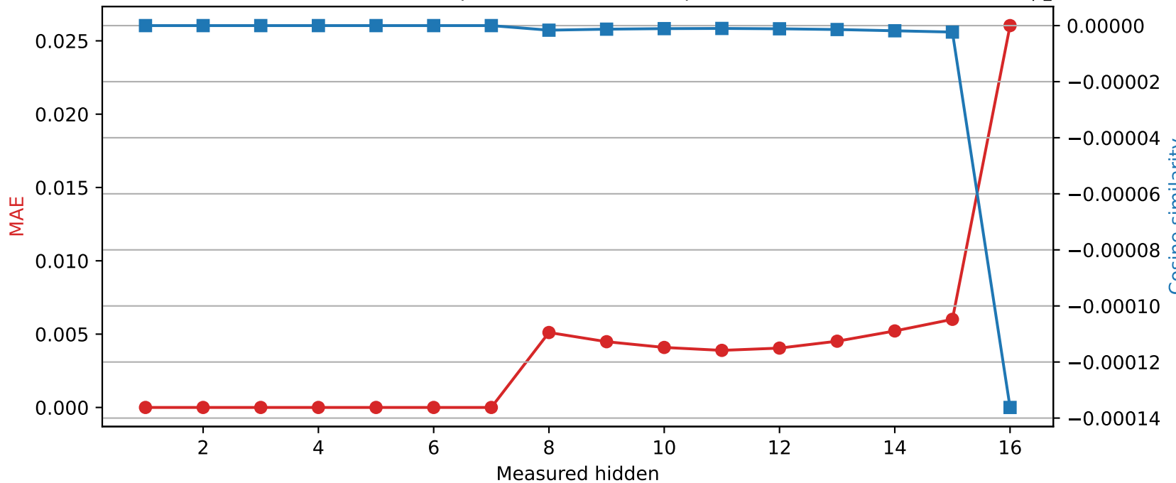
Llama-3.2-1B | Quantized layer 7 | float64 → int8
