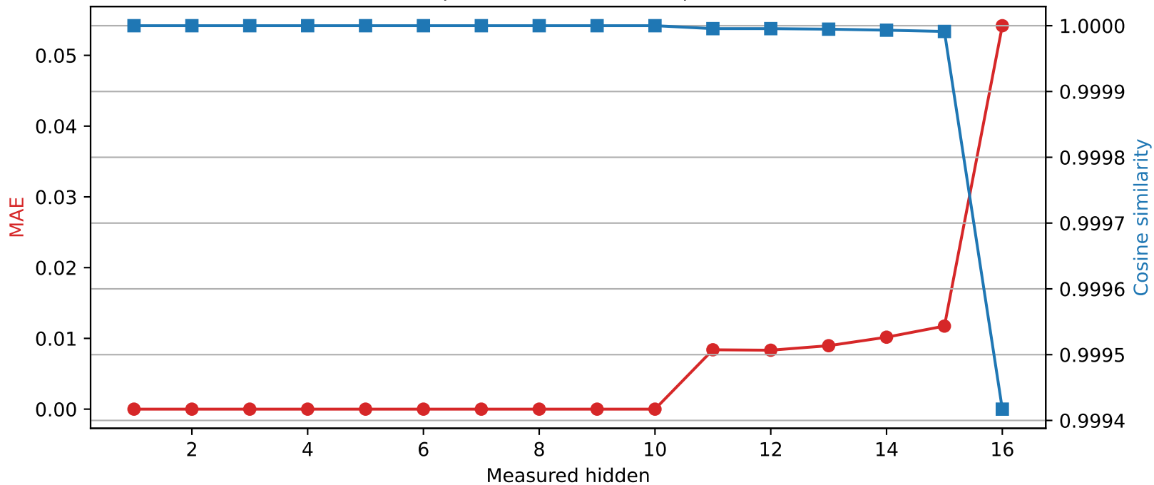
Llama-3.2-1B | Quantized layer 10 | float64 → int8
