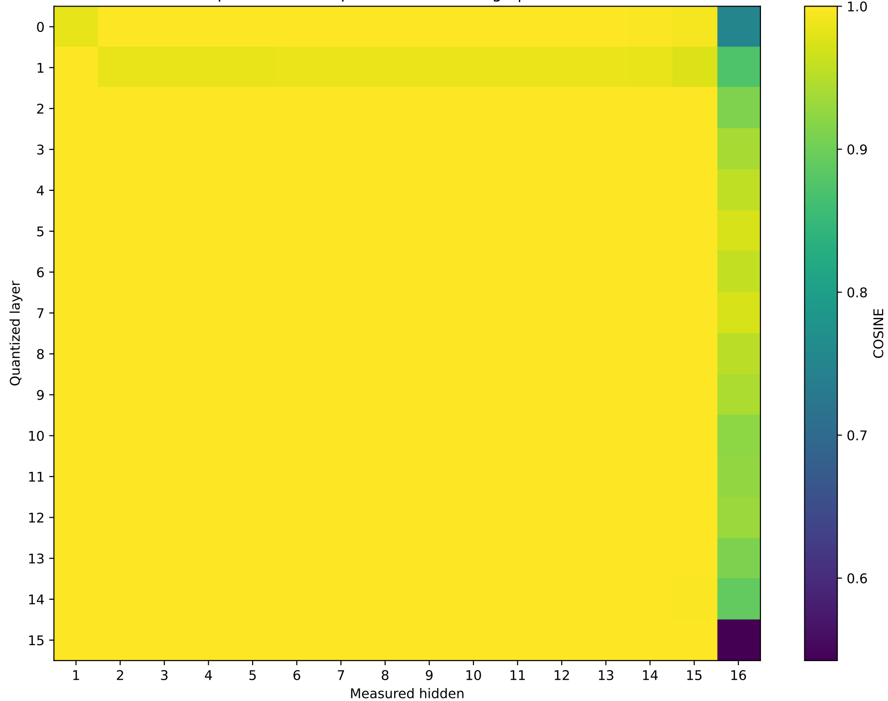
Llama-3.2-1B Prompt 0: cos sim representation damage | float16 → int4
