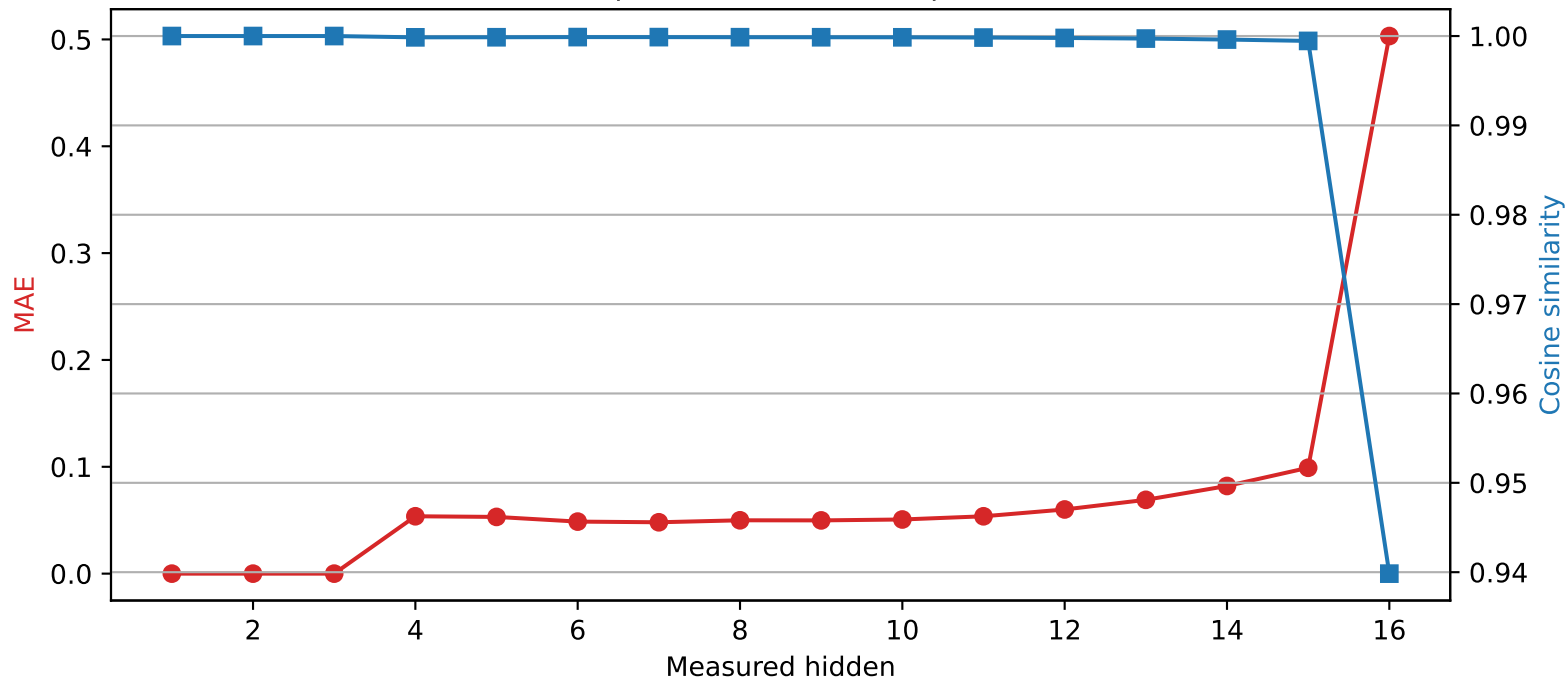
Llama-3.2-1B | Quantized layer 3 | float32 → int4
