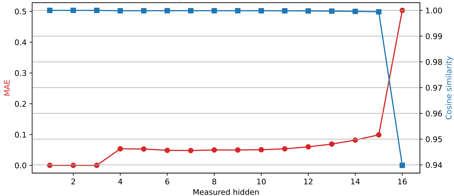
Llama-3.2-1B | Quantized layer 3 | float64 → int4
