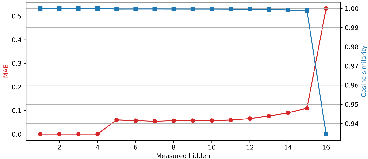
Llama-3.2-1B | Quantized layer 4 | float64 → int4
