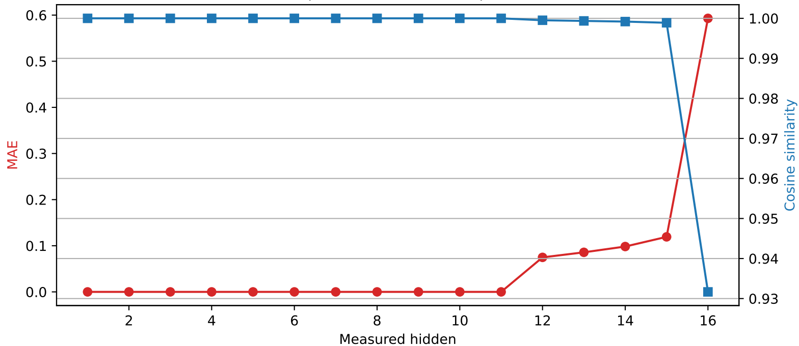
Llama-3.2-1B | Quantized layer 11 | float64 → int4
