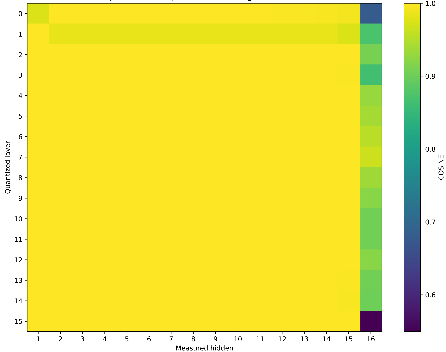
Llama-3.2-1B Prompt 2: cos sim representation damage | float64 → int4
