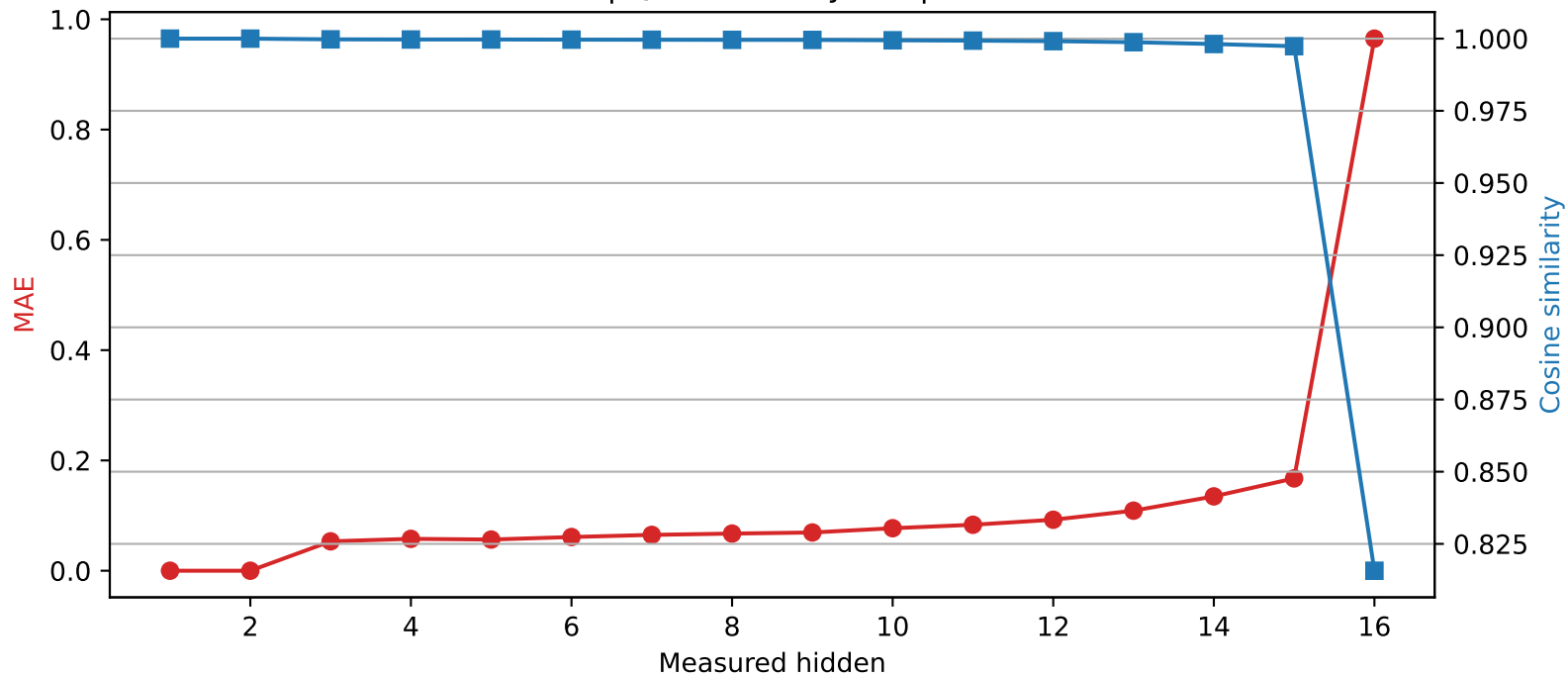
Llama-3.2-1B | Quantized layer 2 | float64 → int4
