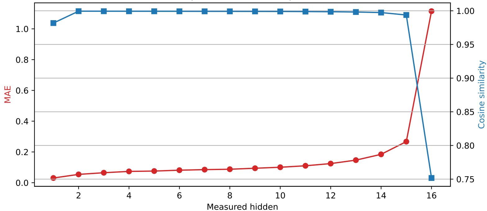
Llama-3.2-1B | Quantized layer 0 | float64 → int4
