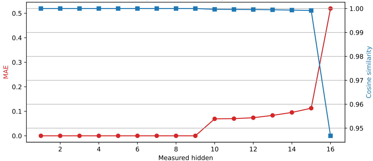
Llama-3.2-1B | Quantized layer 9 | float64 → int4
