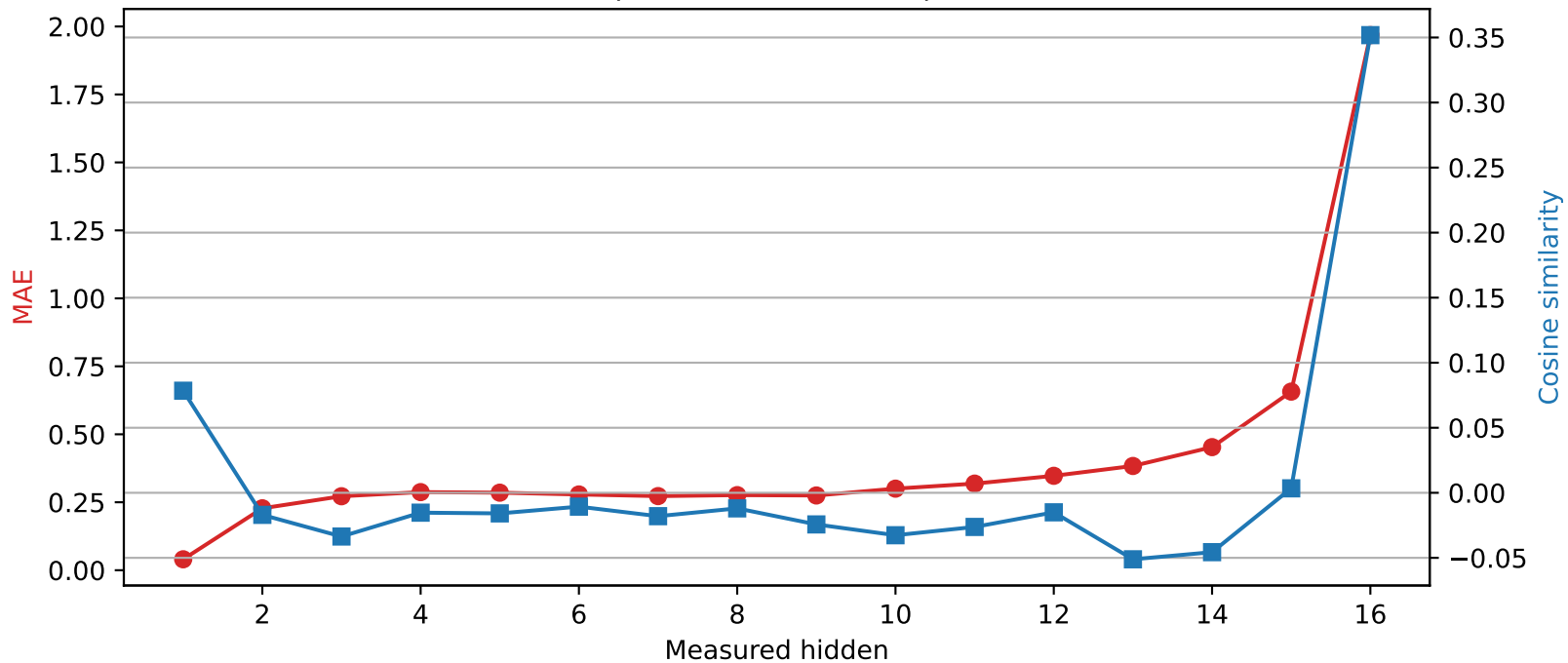
Llama-3.2-1B | Quantized layer 0 | float64 → int2
