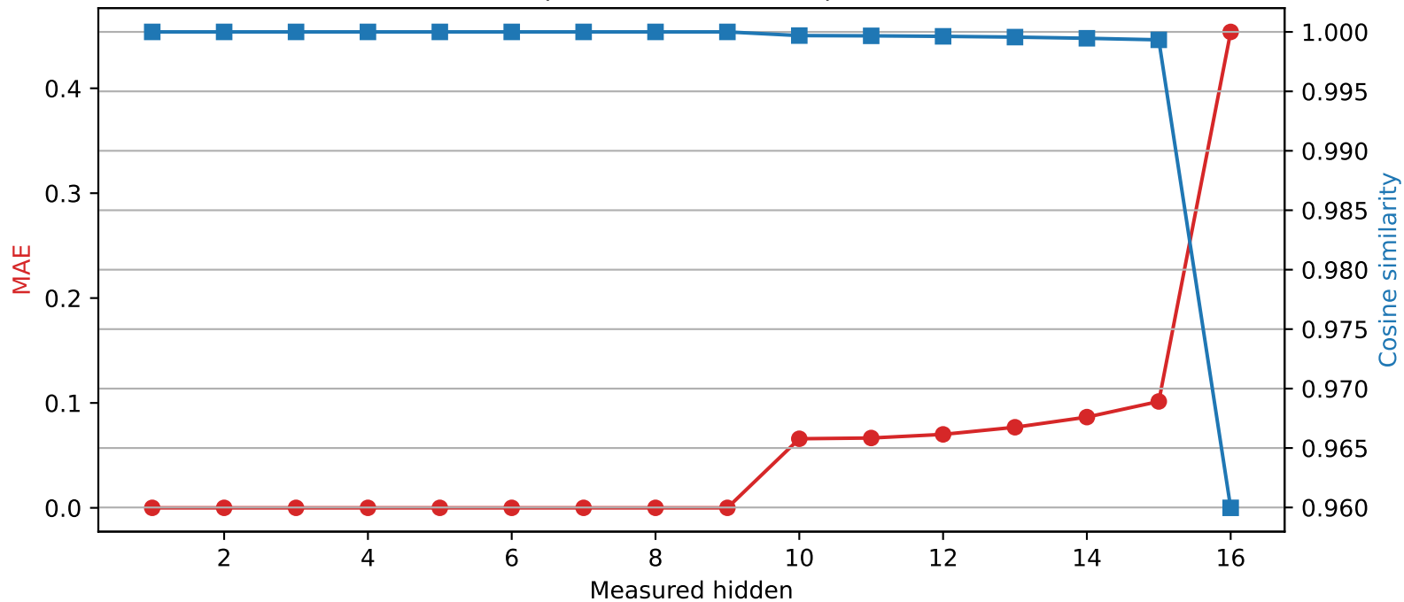
Llama-3.2-1B | Quantized layer 9 | float64 → int2
