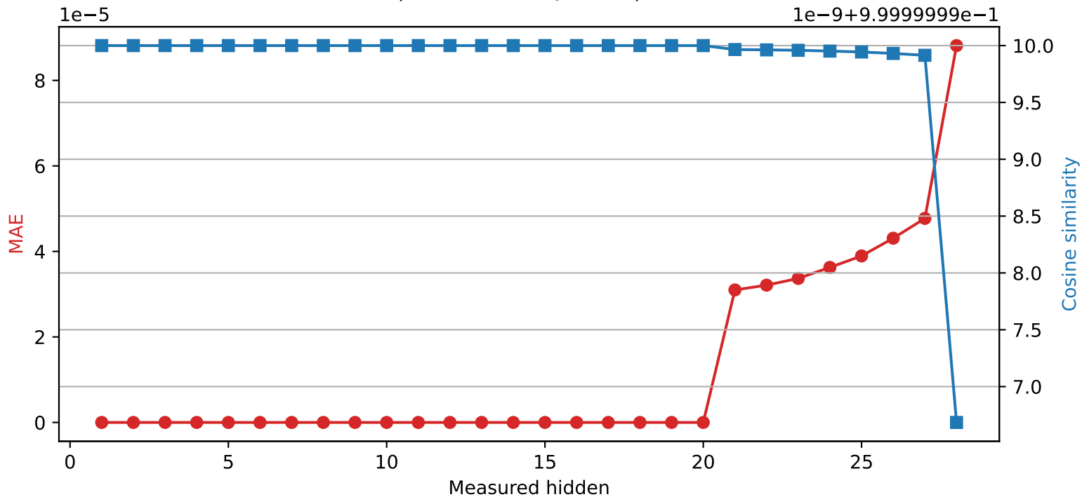
Llama-3.2-3B | Quantized layer 20 | float32 → int16
