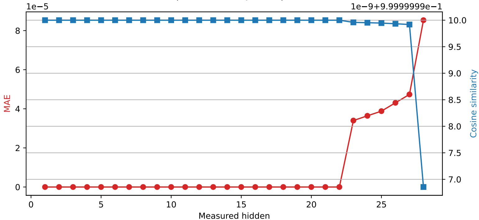
Llama-3.2-3B | Quantized layer 22 | float32 \rightarrow int16
