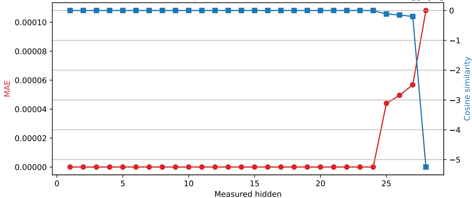
Llama-3.2-3B | Quantized layer 24 | float32 → int16
