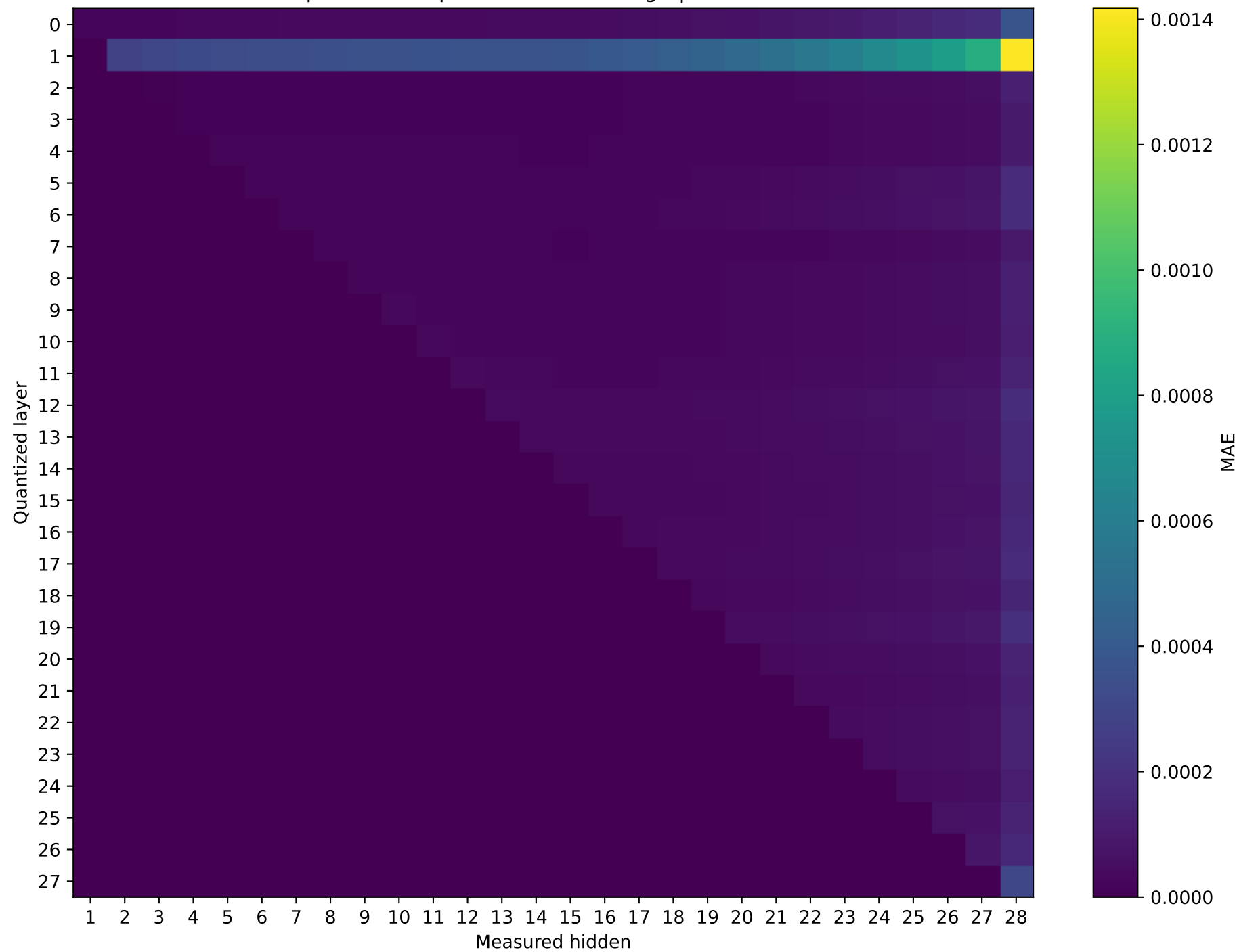
Llama-3.2-3B Prompt 2: MAE representation damage | float32 → int16
