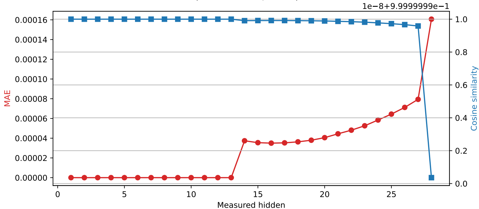
Llama-3.2-3B | Quantized layer 13 | float32 \rightarrow int16
