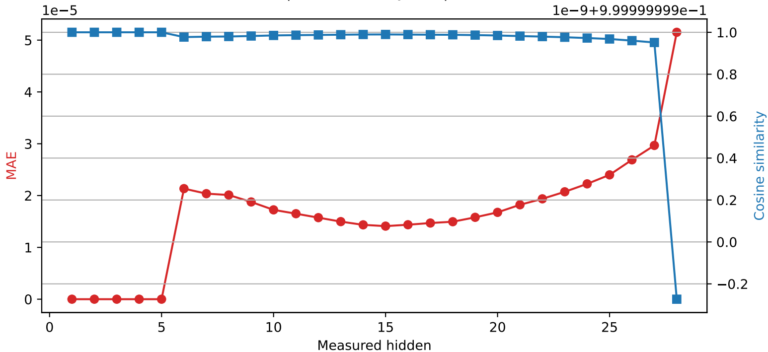
Llama-3.2-3B | Quantized layer 5 | float32 → int16
