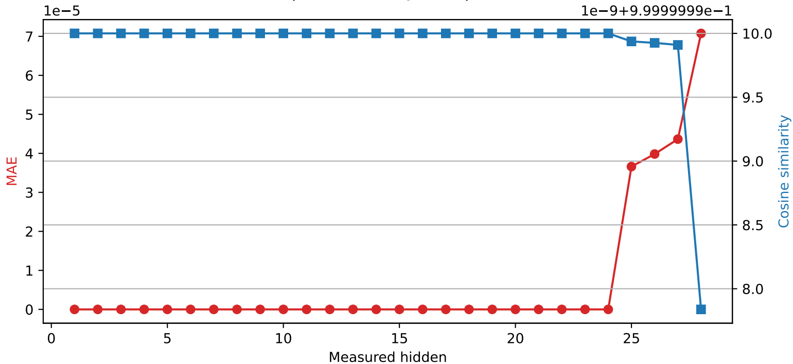
Llama-3.2-3B | Quantized layer 24 | float32 \rightarrow int16
