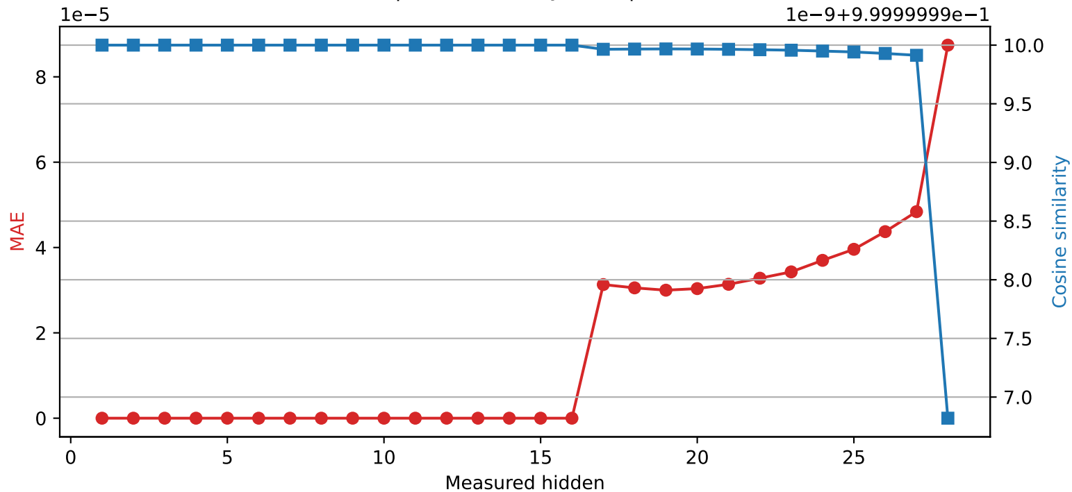
Llama-3.2-3B | Quantized layer 16 | float64 → int16
