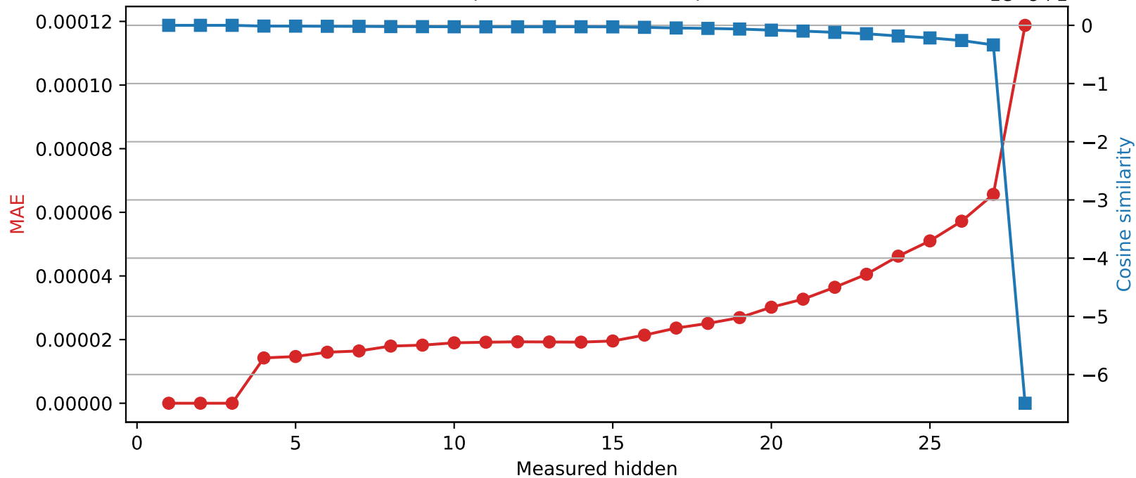
Llama-3.2-3B | Quantized layer 3 | float64 → int16
