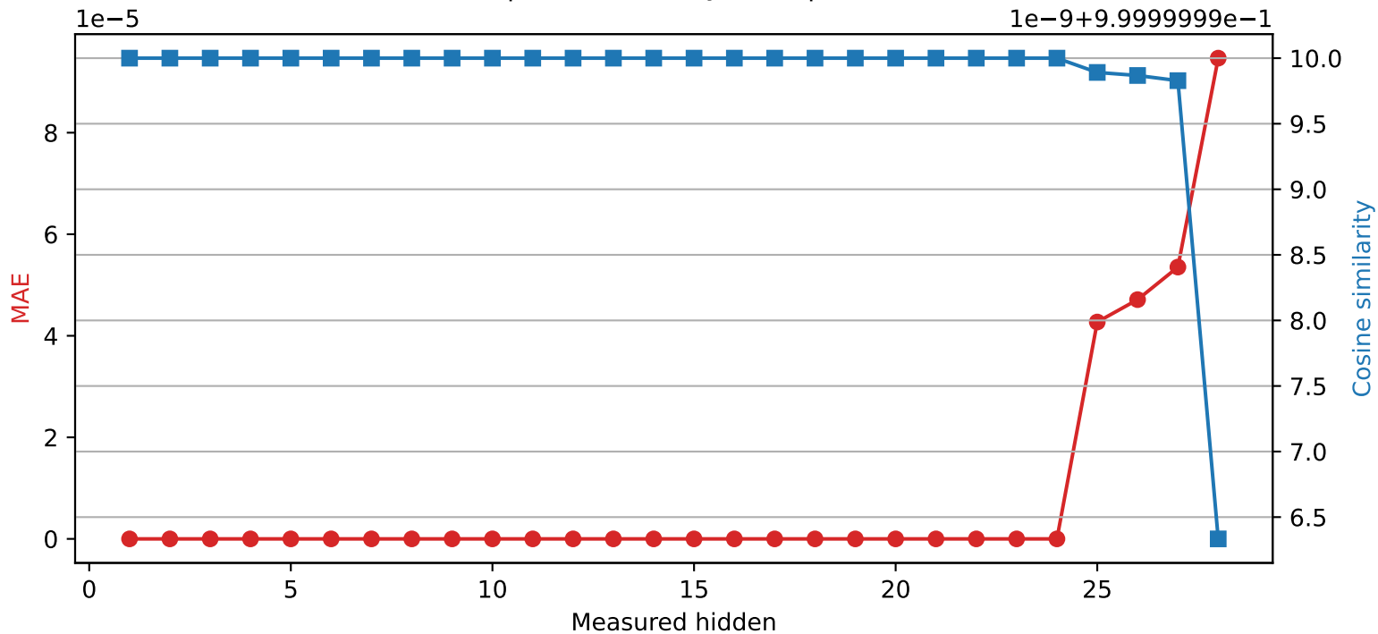
Llama-3.2-3B | Quantized layer 24 | float64 → int16
