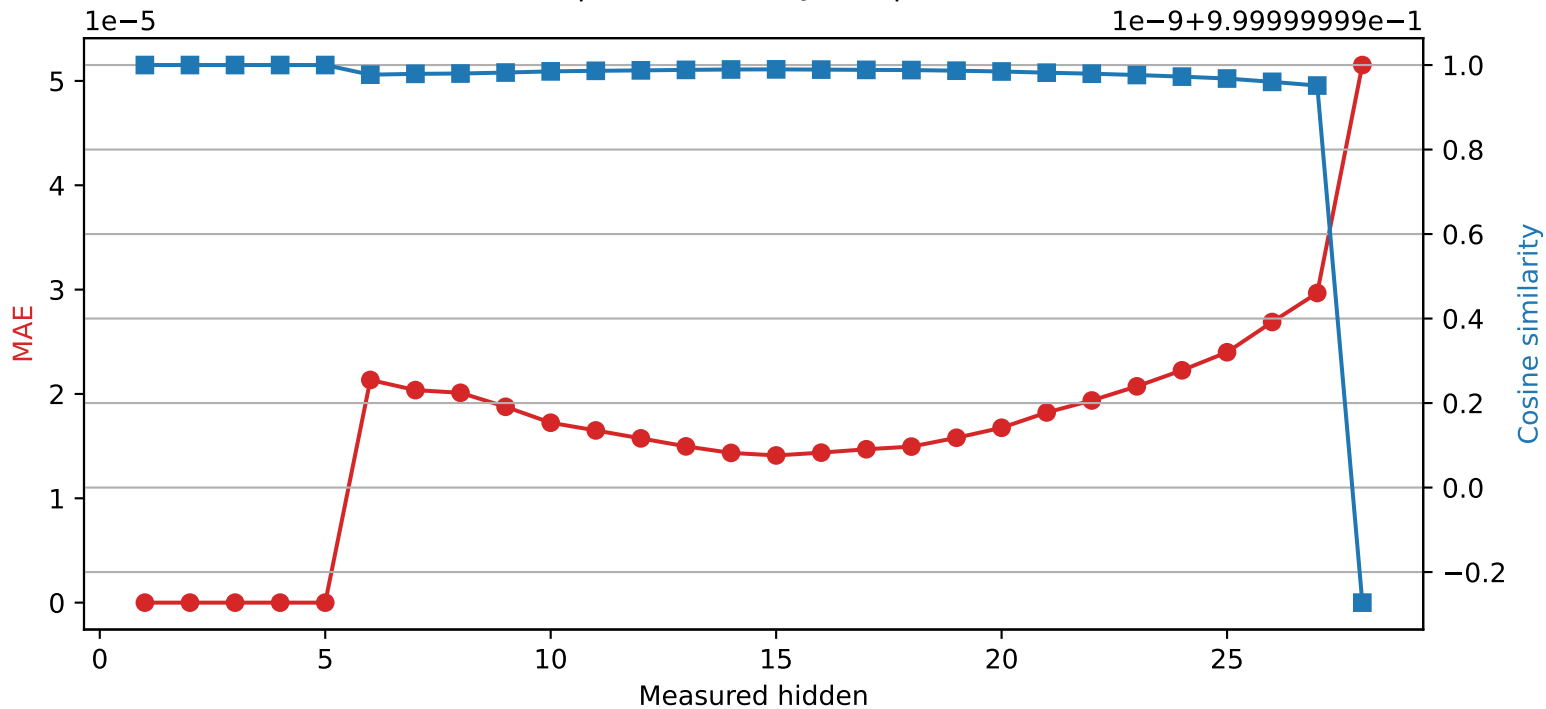
Llama-3.2-3B | Quantized layer 5 | float64 → int16
