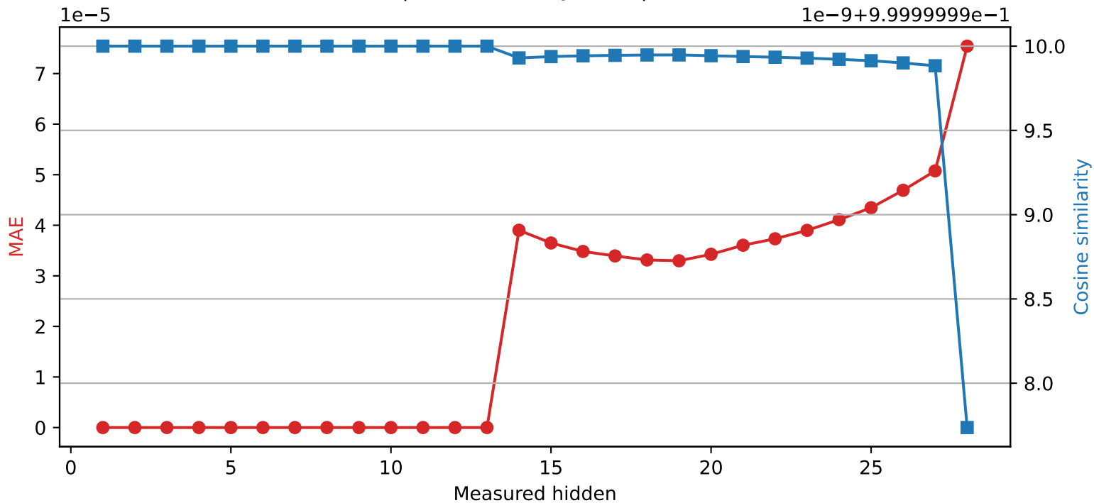
Llama-3.2-3B | Quantized layer 13 | float64 → int16
