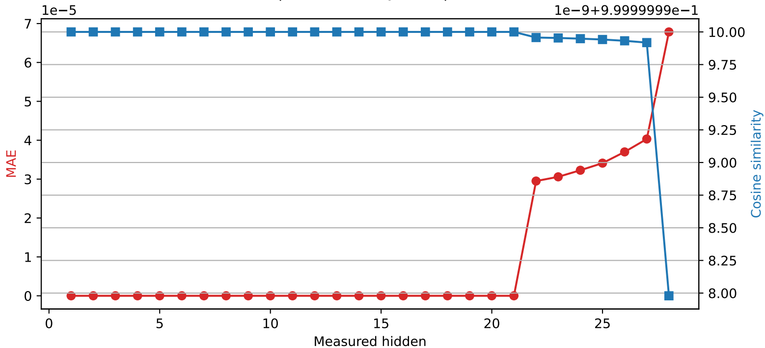
Llama-3.2-3B | Quantized layer 21 | float64 → int16
