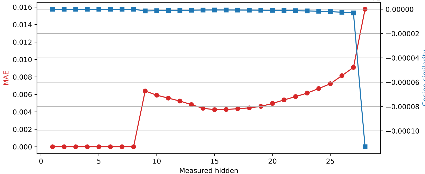
Llama-3.2-3B | Quantized layer 8 | float16 → int8
