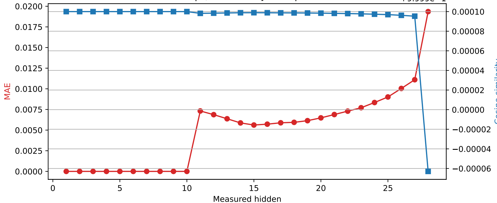
Llama-3.2-3B | Quantized layer 10 | float16 → int8
