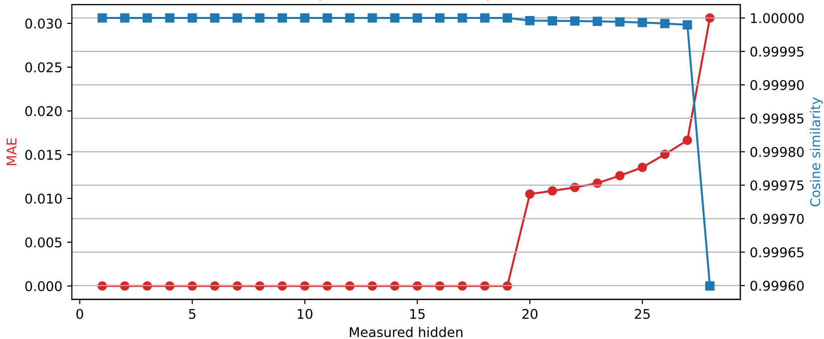
Llama-3.2-3B | Quantized layer 19 | float16 → int8
