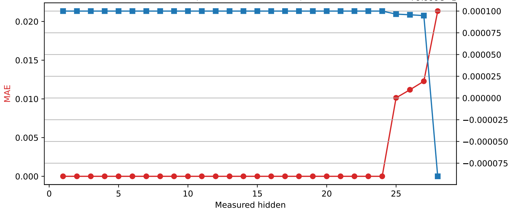
Llama-3.2-3B | Quantized layer 24 | float16 → int8
