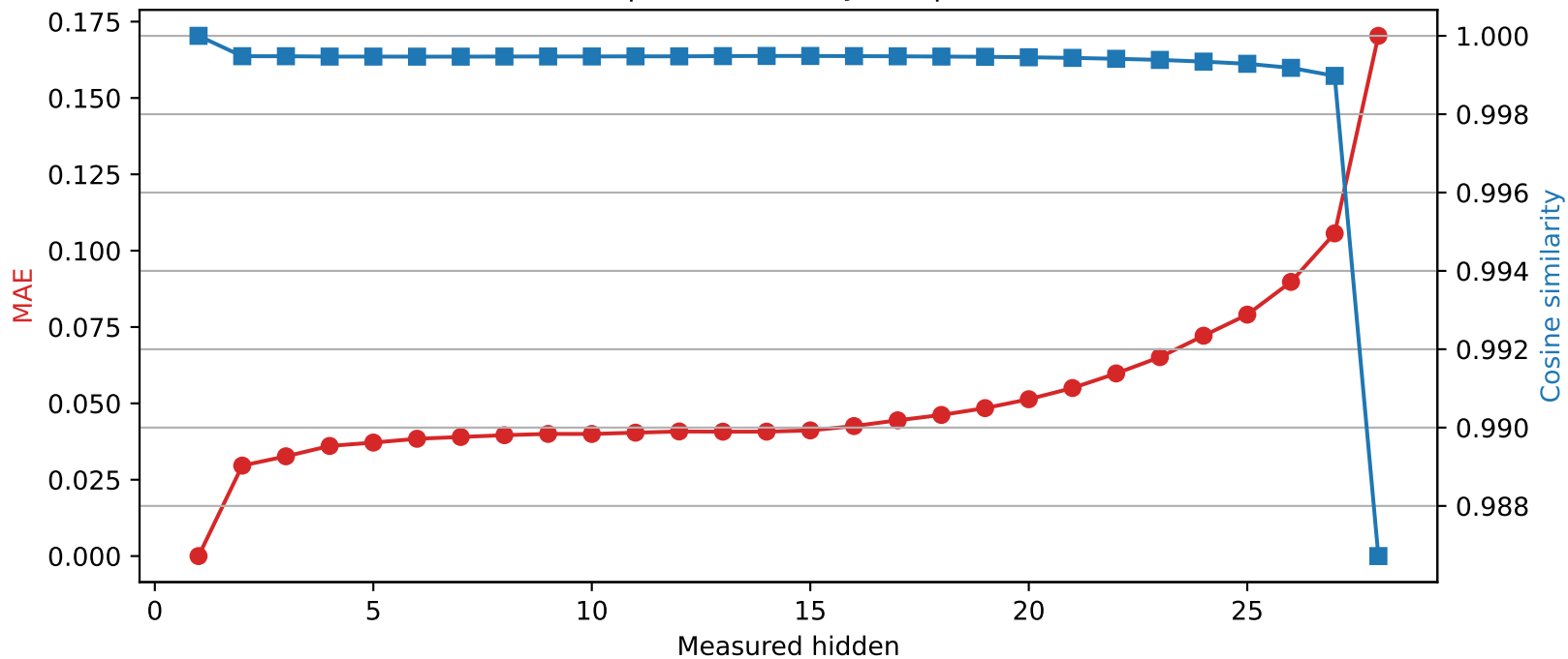
Llama-3.2-3B | Quantized layer 1 | float16 → int8
