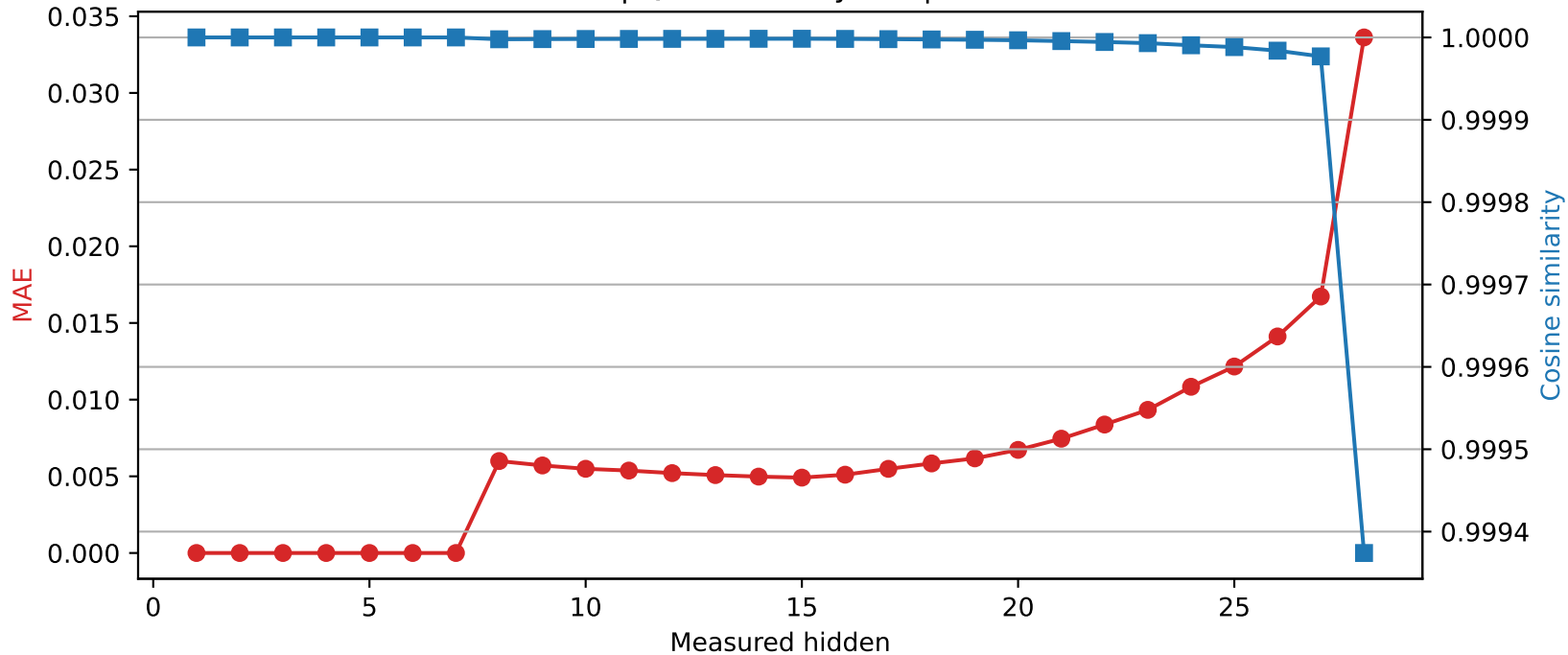
Llama-3.2-3B | Quantized layer 7 | float16 \rightarrow int8
