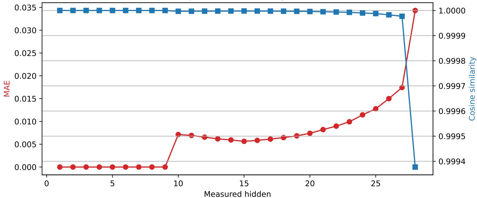
Llama-3.2-3B | Quantized layer 9 | float16 \rightarrow int8
