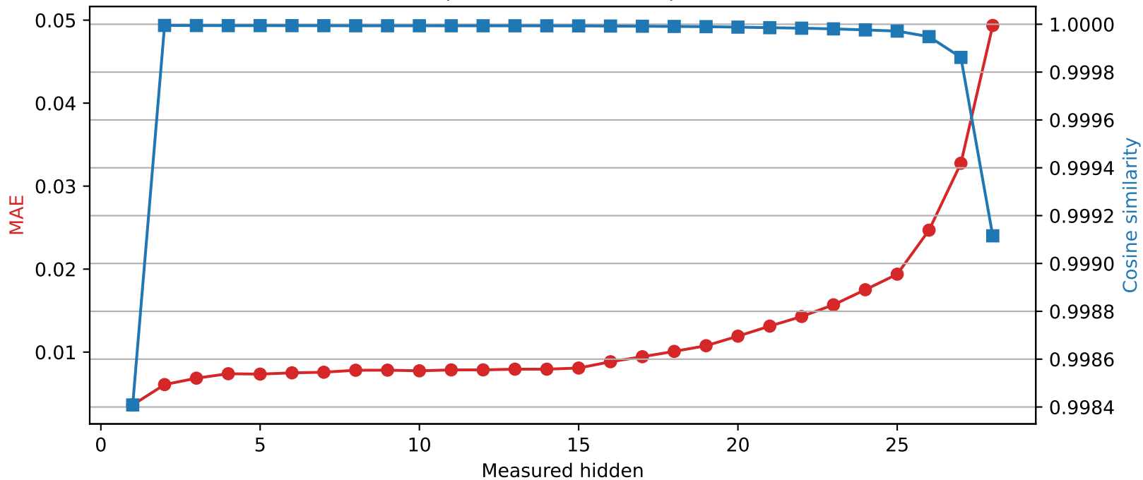
Llama-3.2-3B | Quantized layer 0 | float16 \rightarrow int8
