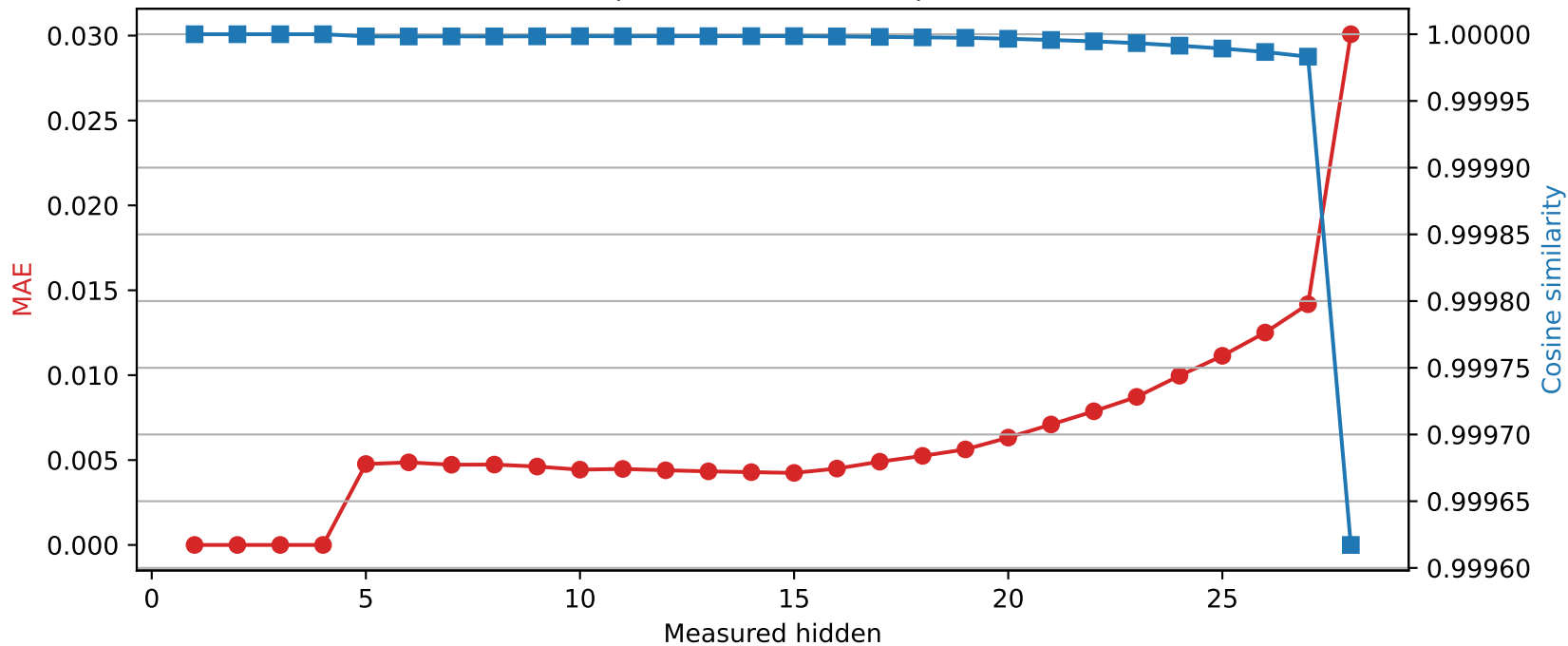
Llama-3.2-3B | Quantized layer 4 | float16 → int8
