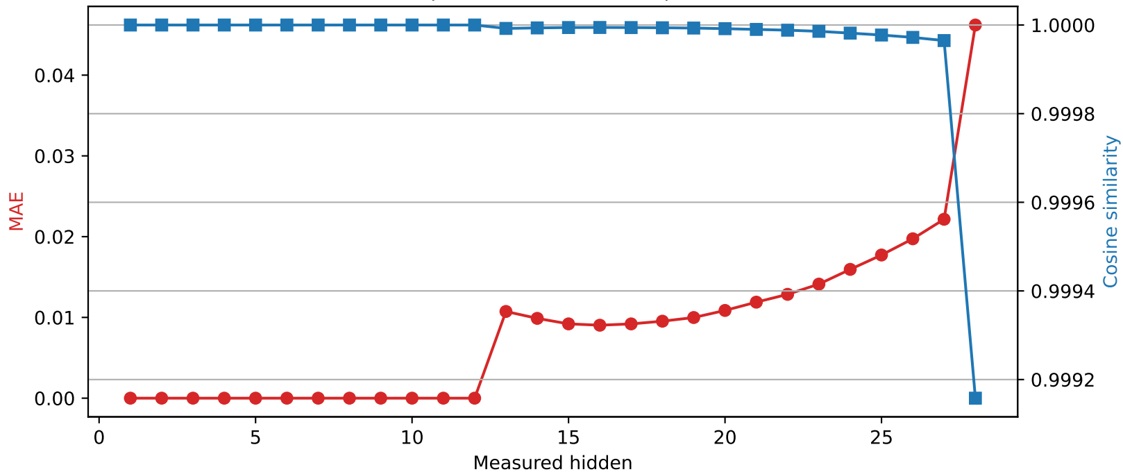
Llama-3.2-3B | Quantized layer 12 | float16 \rightarrow int8
