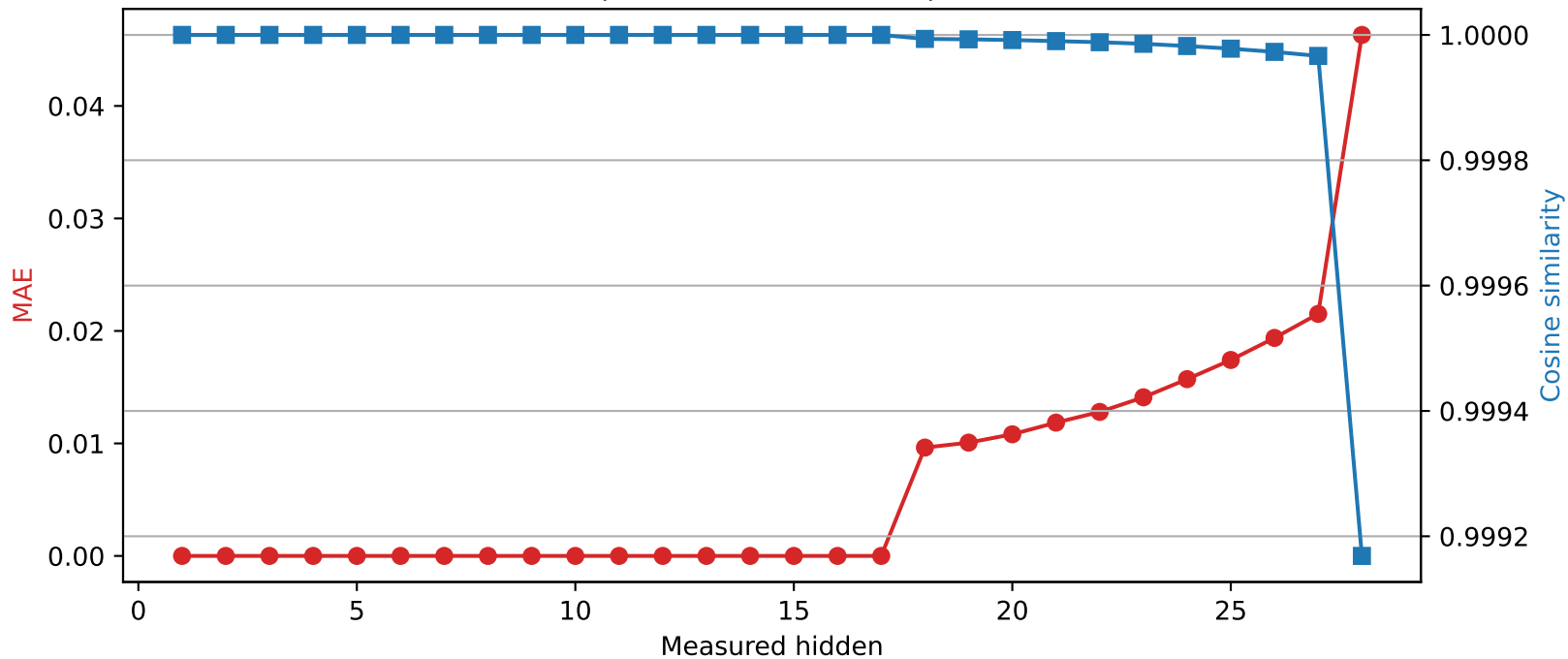
Llama-3.2-3B | Quantized layer 17 | float16 \rightarrow int8
