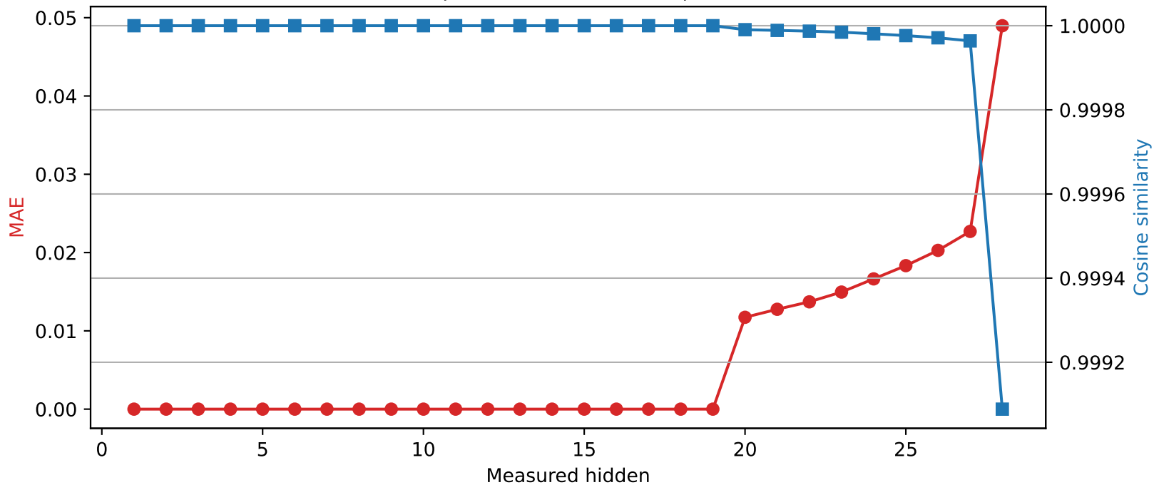
Llama-3.2-3B | Quantized layer 19 | float16 \rightarrow int8
