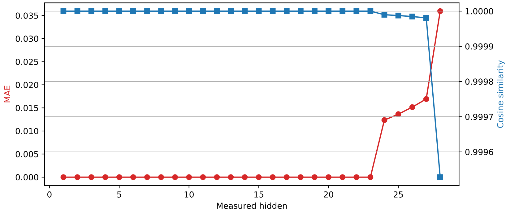
Llama-3.2-3B | Quantized layer 23 | float16 \rightarrow int8
