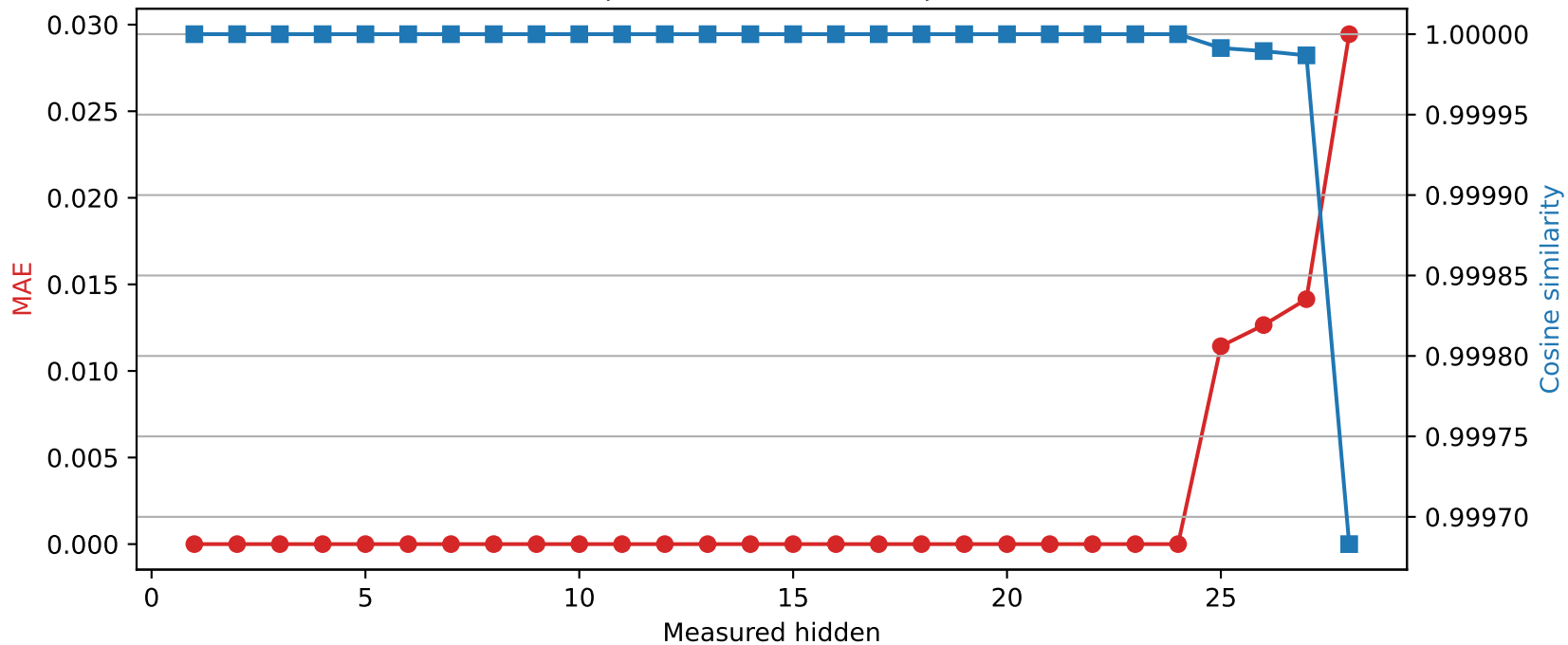
Llama-3.2-3B | Quantized layer 24 | float16 \rightarrow int8
