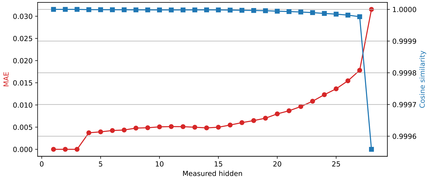
Llama-3.2-3B | Quantized layer 3 | float16 \rightarrow int8
