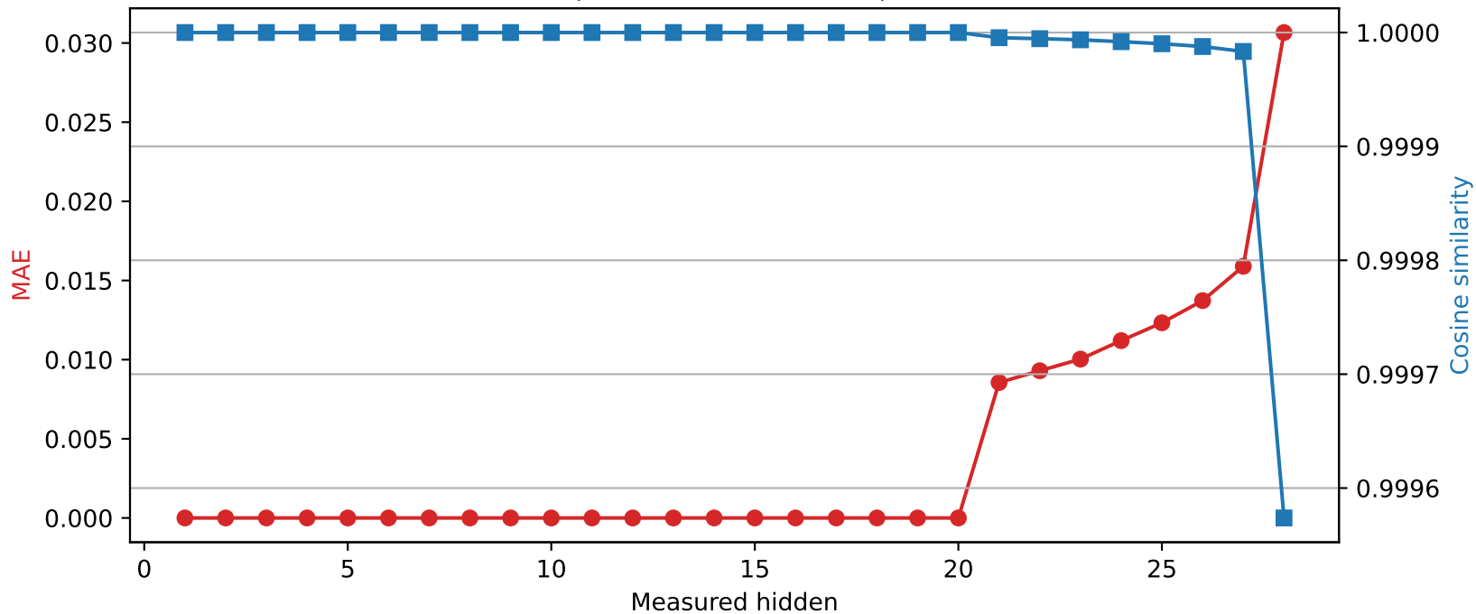
Llama-3.2-3B | Quantized layer 20 | float16 → int8
