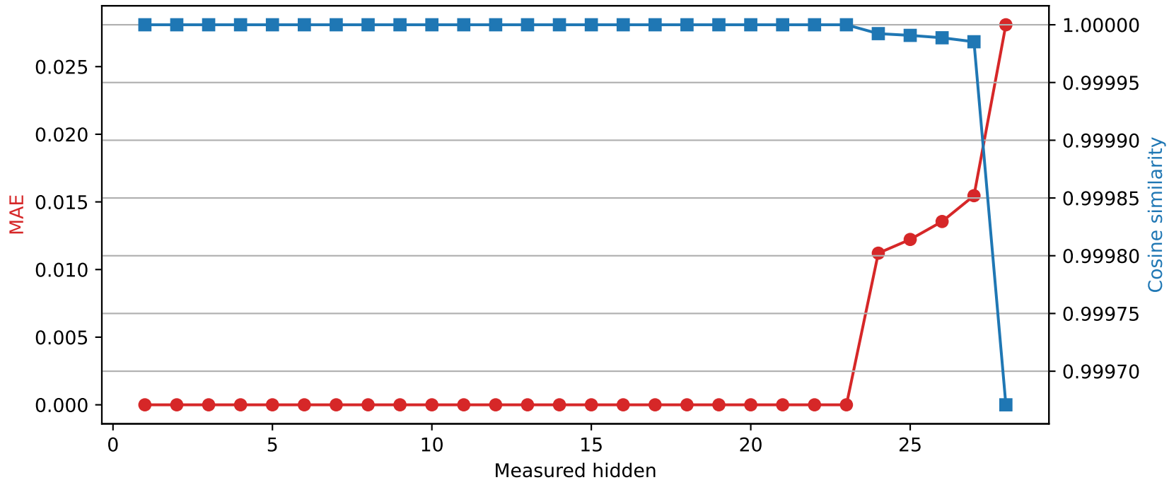
Llama-3.2-3B | Quantized layer 23 | float16 \rightarrow int8
