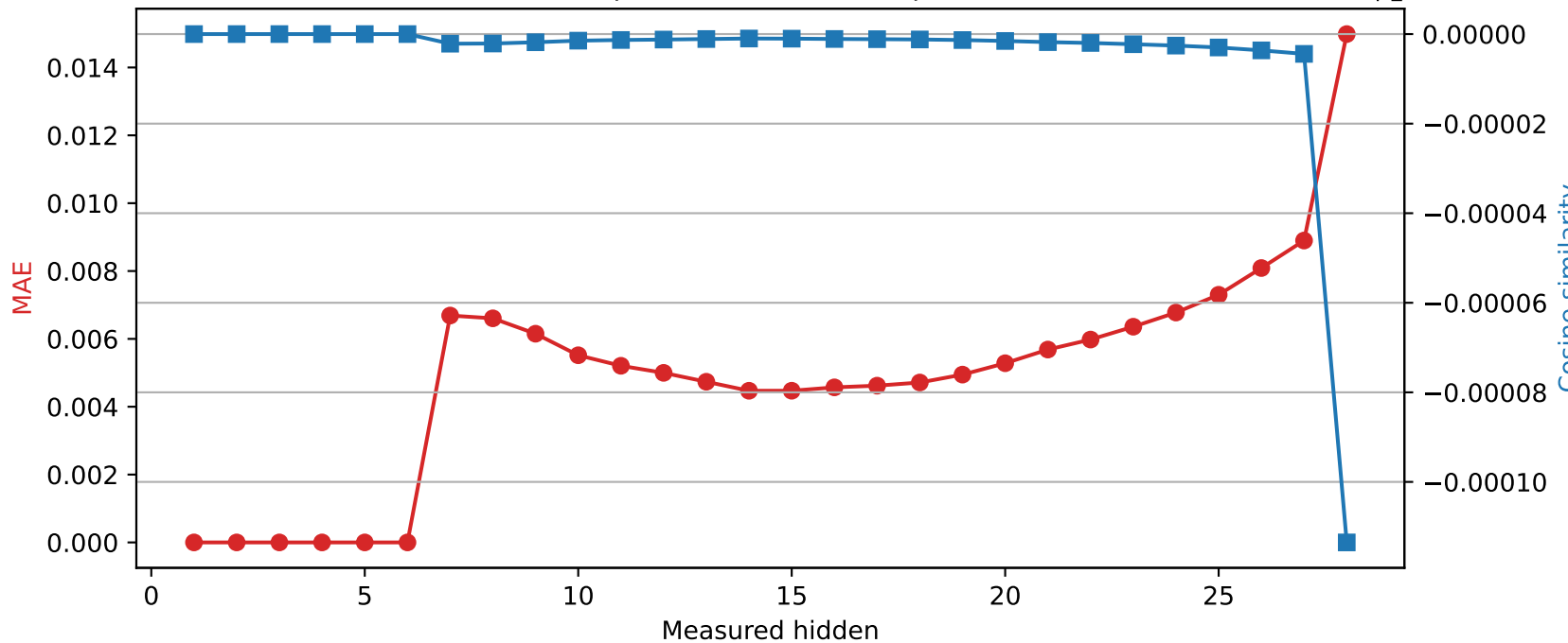
Llama-3.2-3B | Quantized layer 6 | float16 → int8
