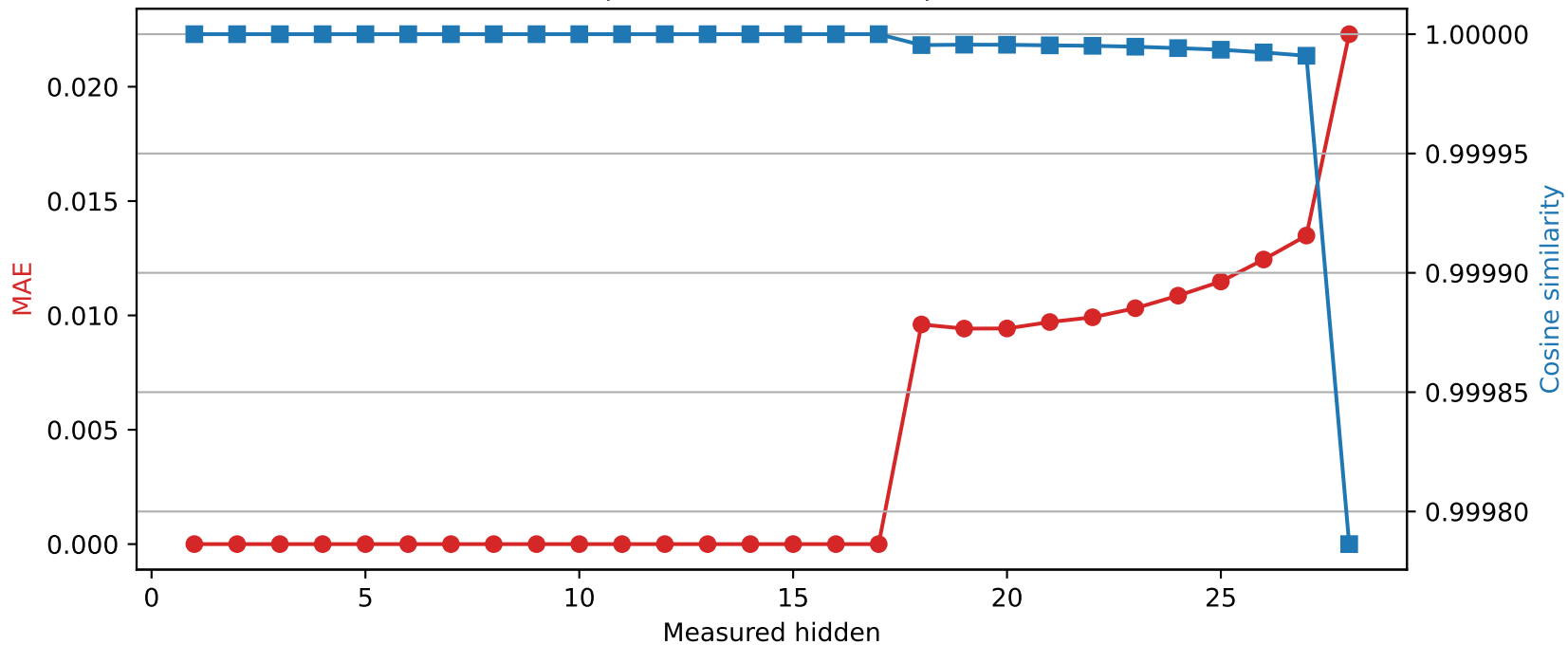
Llama-3.2-3B | Quantized layer 17 | float16 \rightarrow int8
