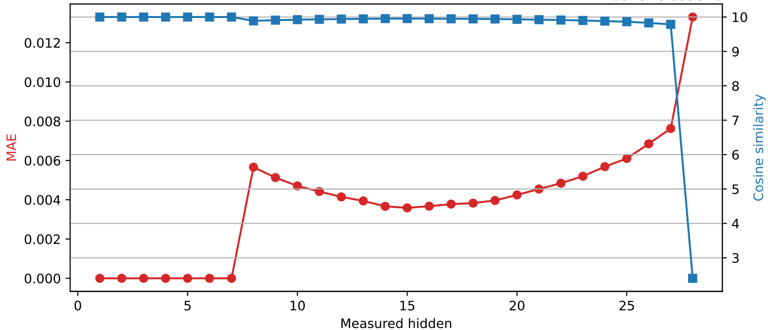
Llama-3.2-3B | Quantized layer 7 | float32 → int8
