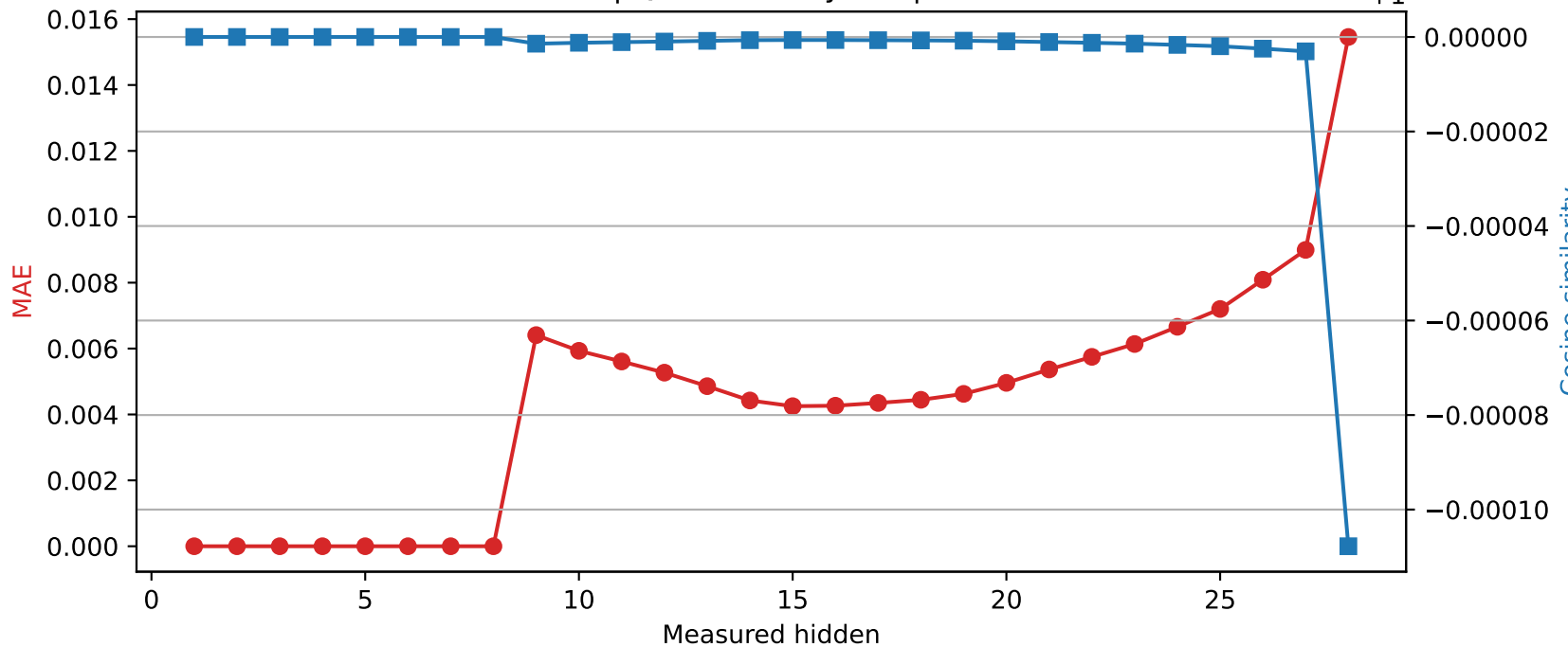
Llama-3.2-3B | Quantized layer 8 | float32 → int8
